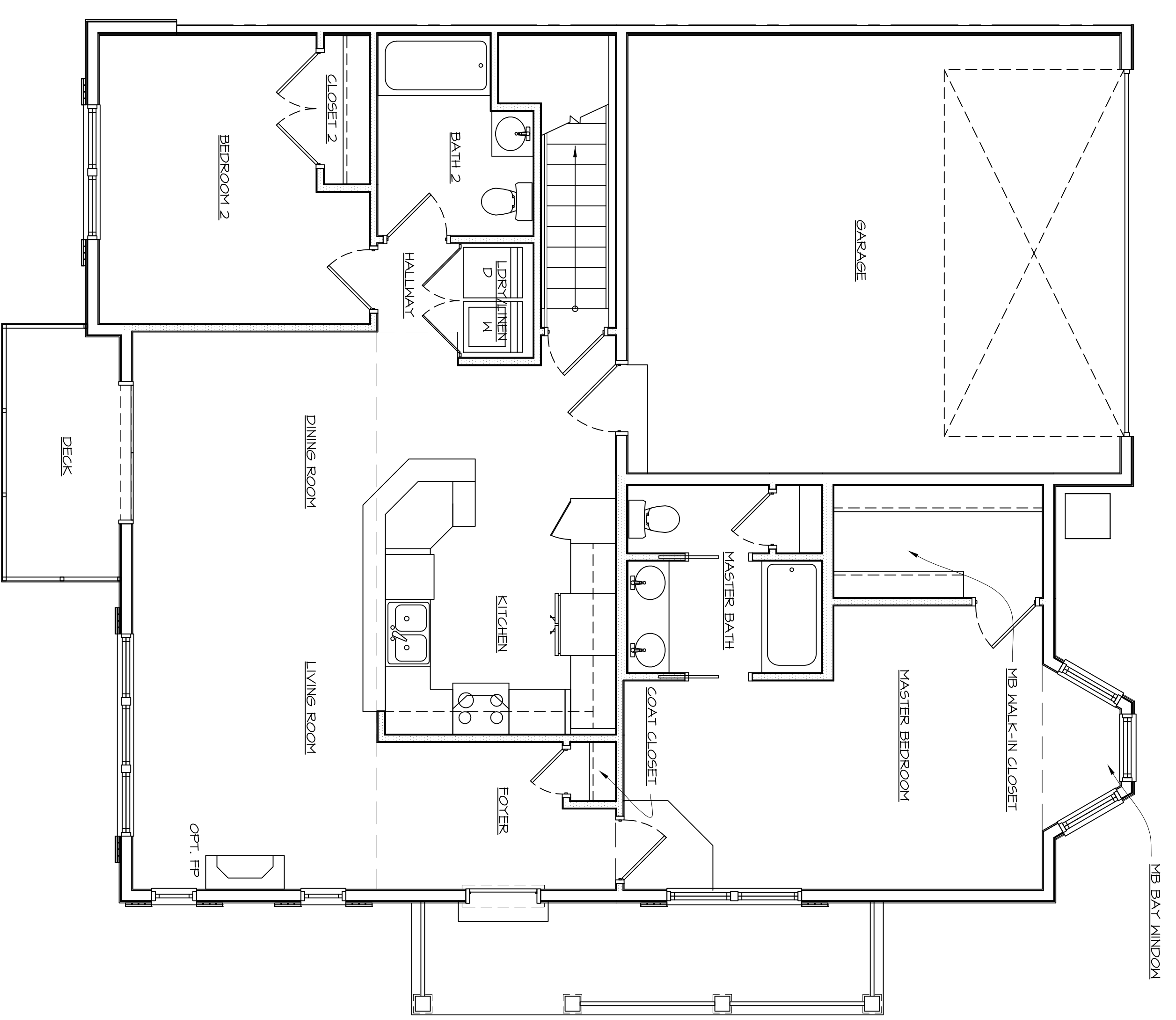
1ST FLOOR FINISHING PLAN
